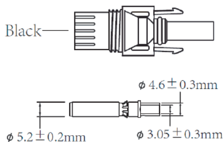
Pic 5.1 DC+ male connector
